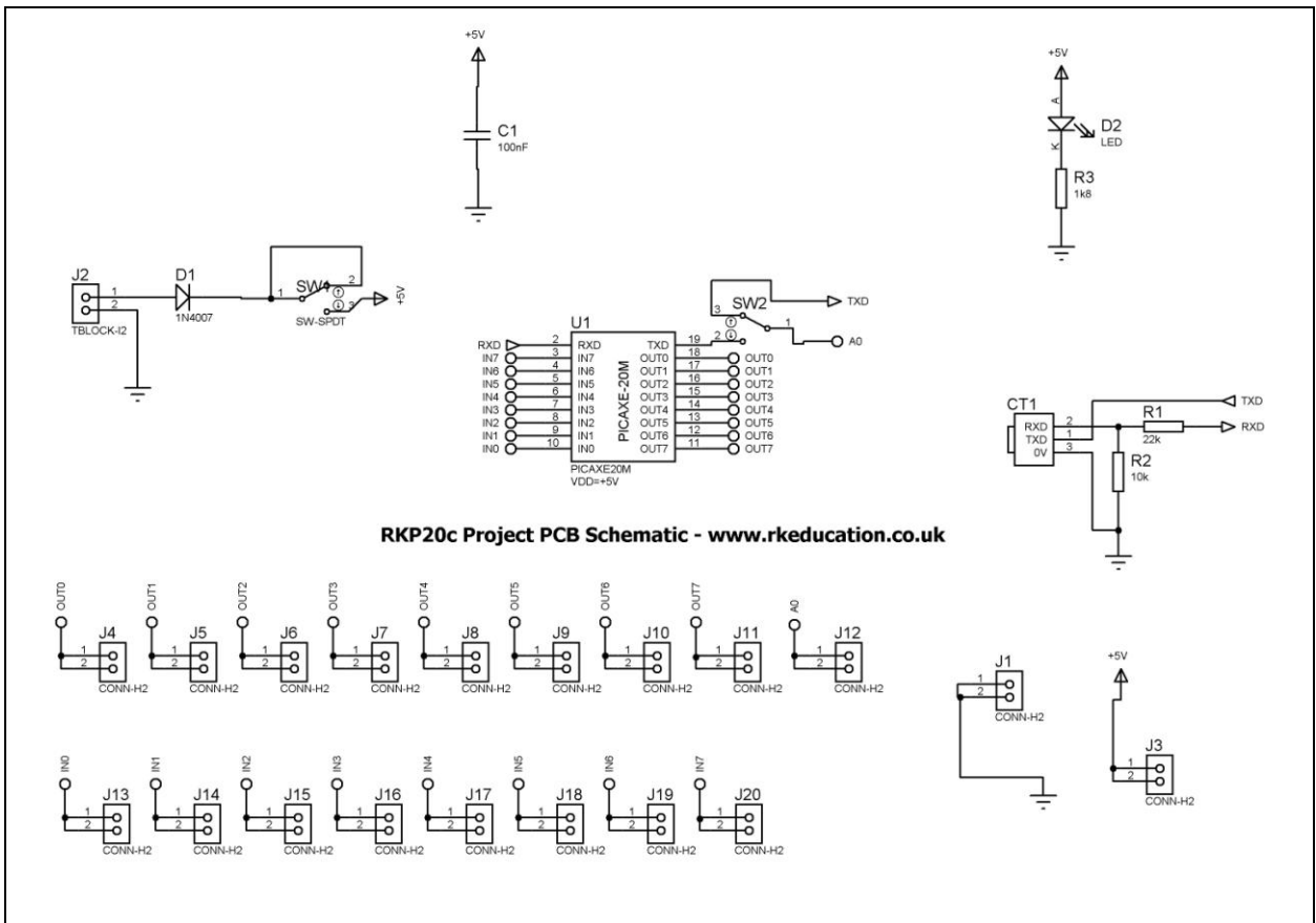
Schematic Diagram
