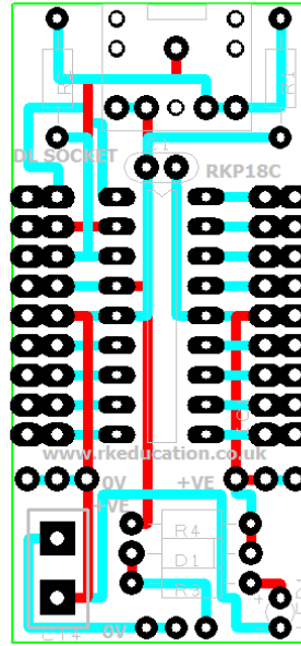
PCB Layout
