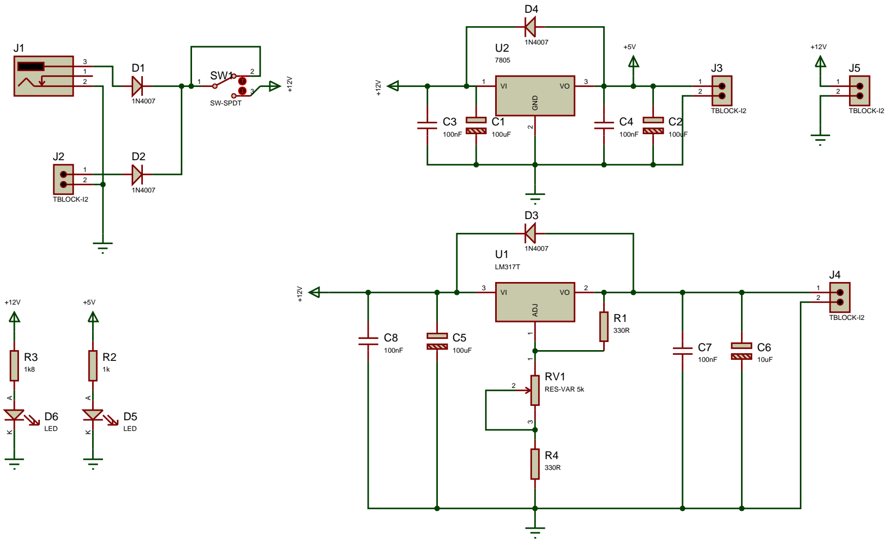
Triple Output PSU Schematic - www.rkeducation.co.uk
