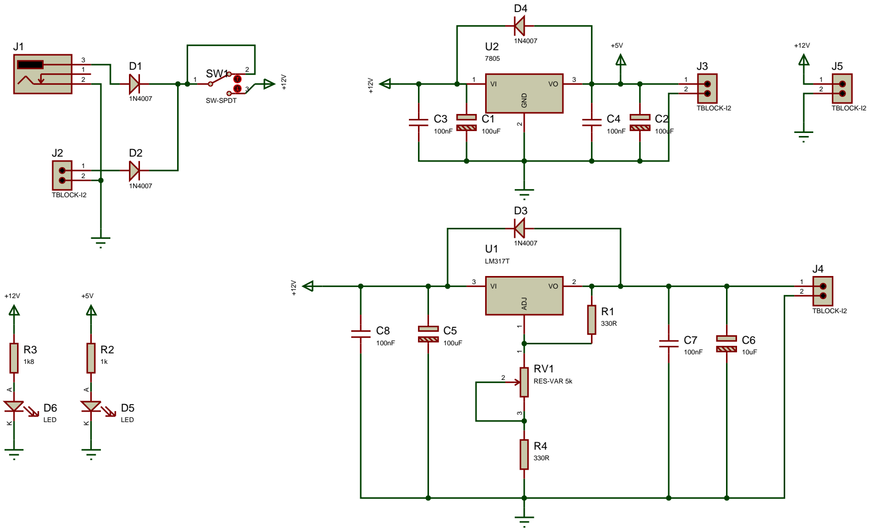
Triple Output PSU Schematic - www.rkeducation.co.uk
