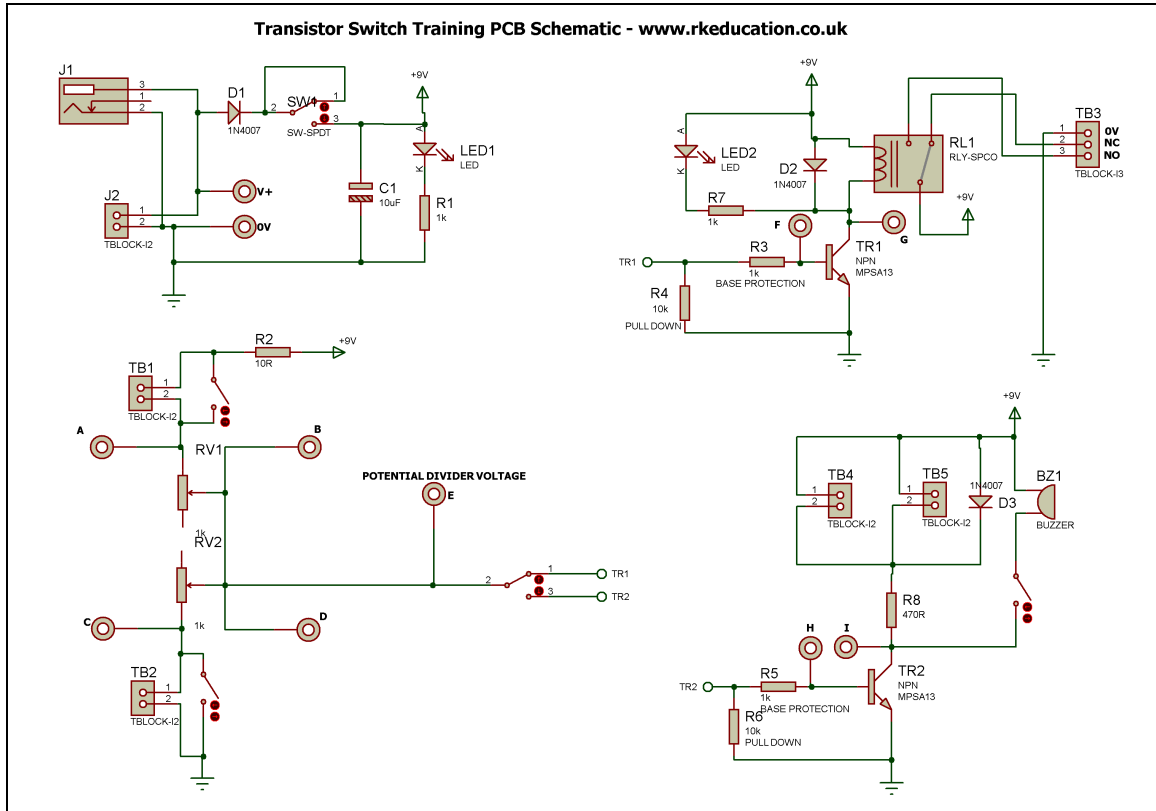
Schematic Diagram
