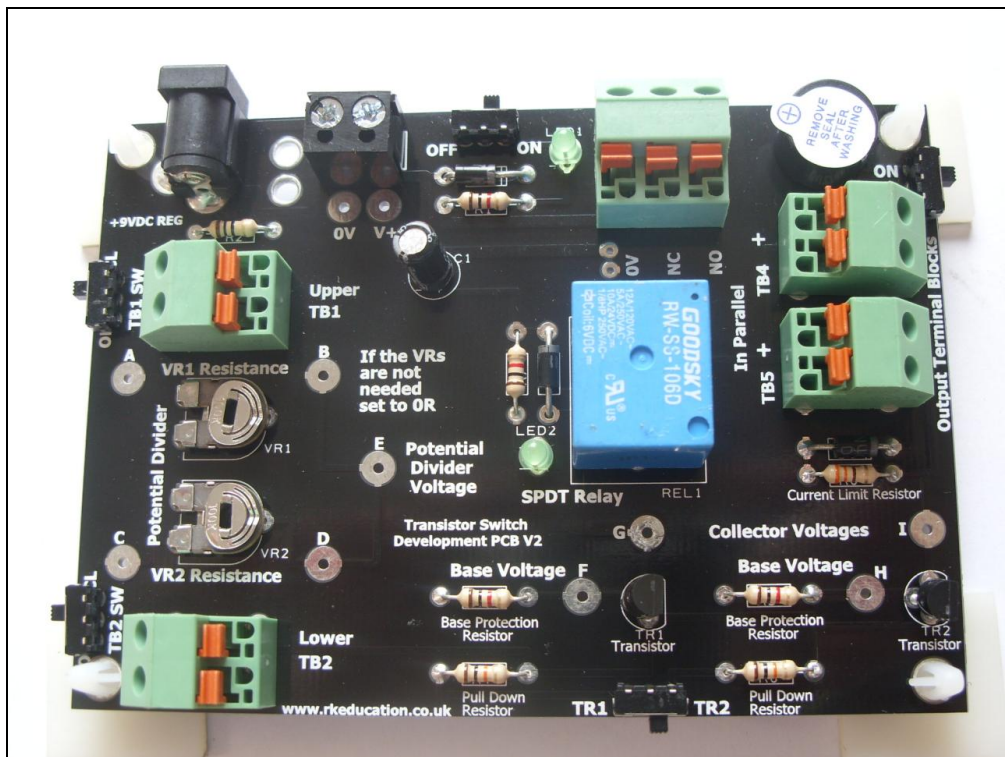
Constructed PCB
