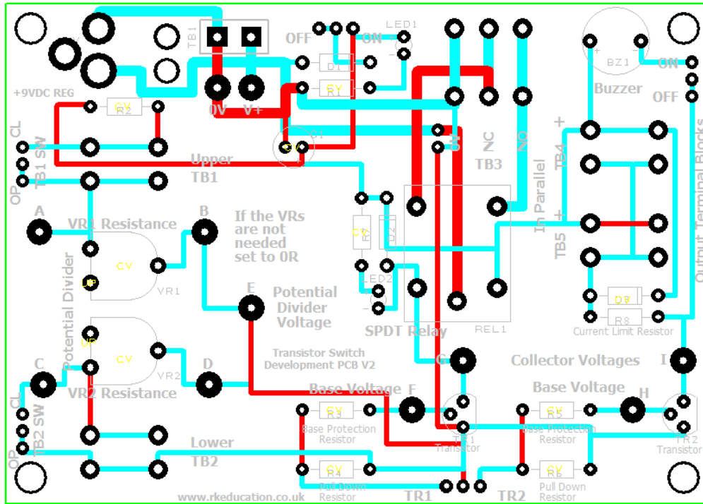
PCB layout
