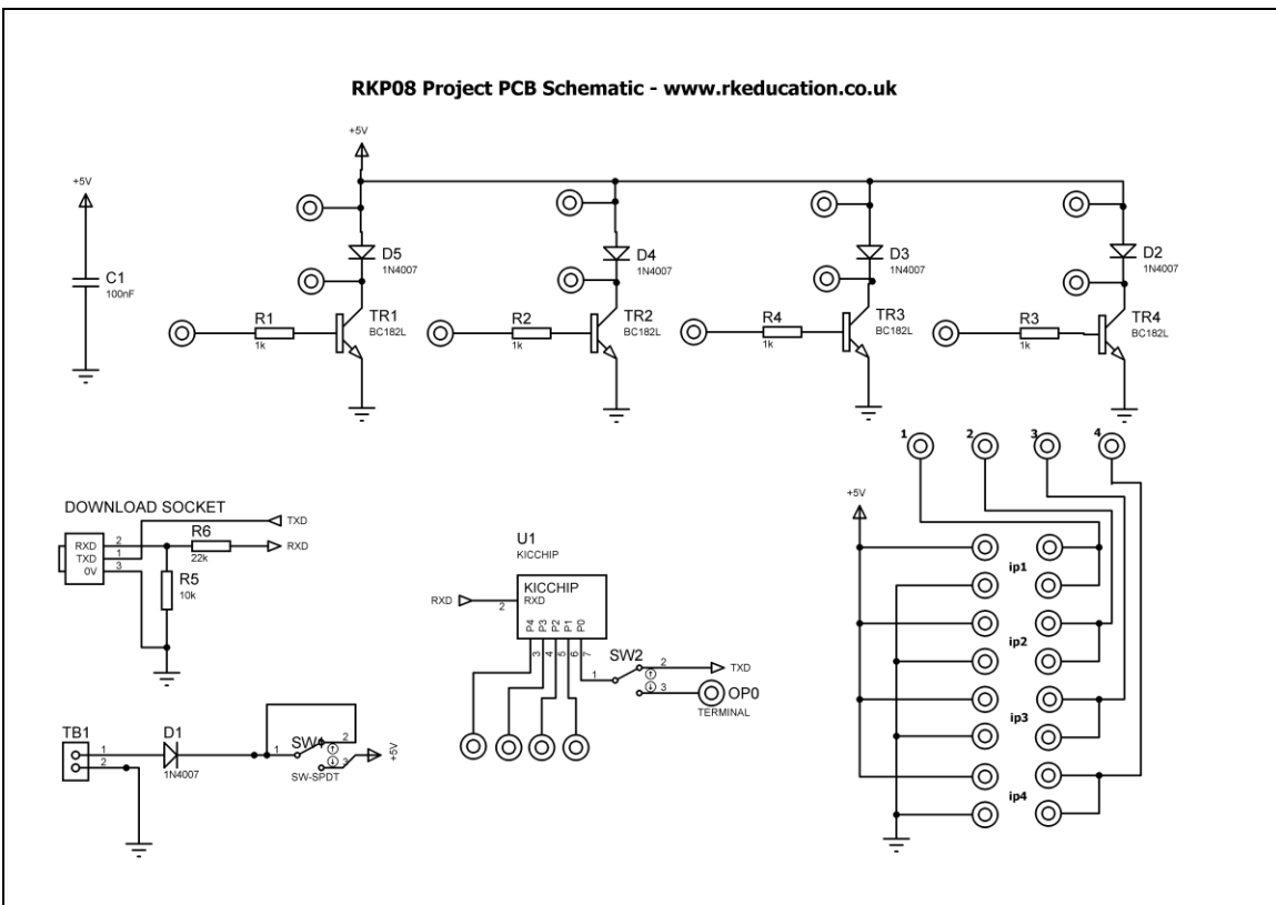
RKP08 Schematic
